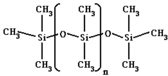
Polydimethylsiloxane
